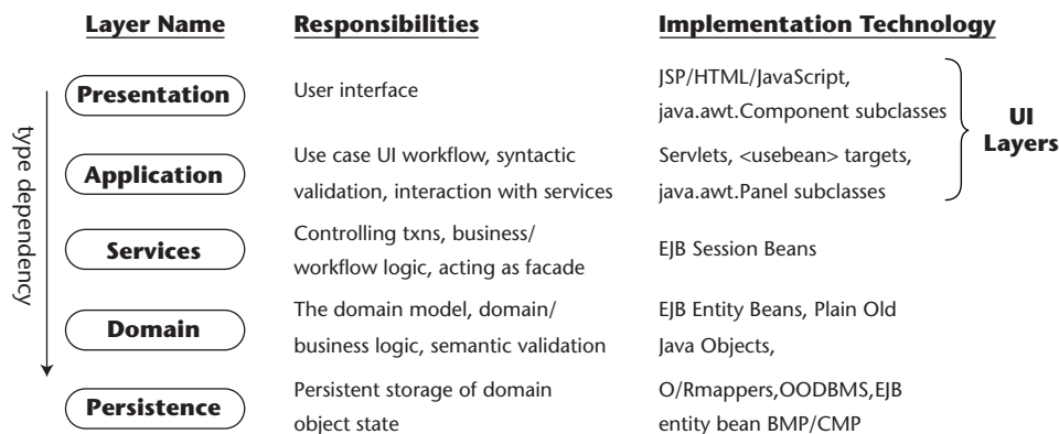
Figure 7.1 Layered architecture.
