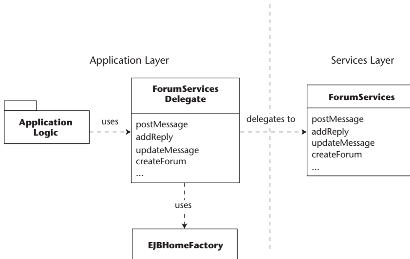
Figure 6.13 Business delegate.
