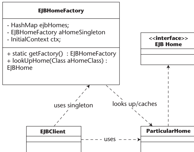
Figure 4.1 EJBHomeFactory implementation.
